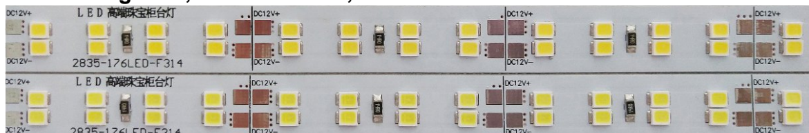
2835 SMD light bar, 176 LEDs/meter, 21W/meter
