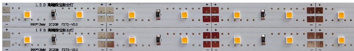
2835 SMD light bar, 176 LEDs/meter, 21W/meter
