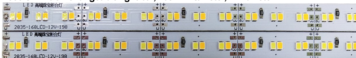
2835 SMD CCT changeable light bar, 168 LEDs/meter, 21W/meter
